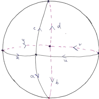
Figure 2: Malcev's condition Z as a spherical axiom
